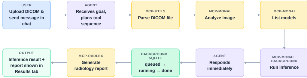
Figure 3: Use Case 1 - Interactive DICOM analysis and segmentation workflow.
