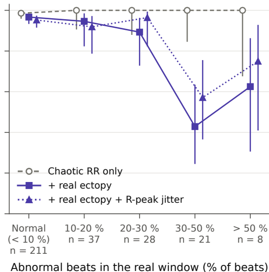
b Logistic map spiked in
