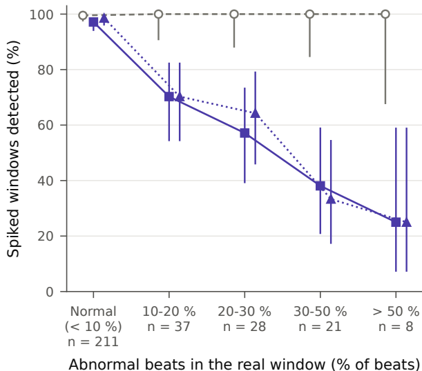
a Hénon map spiked in
