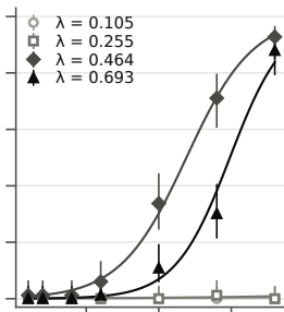
Logistic map
