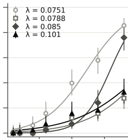
Coupled vdP
