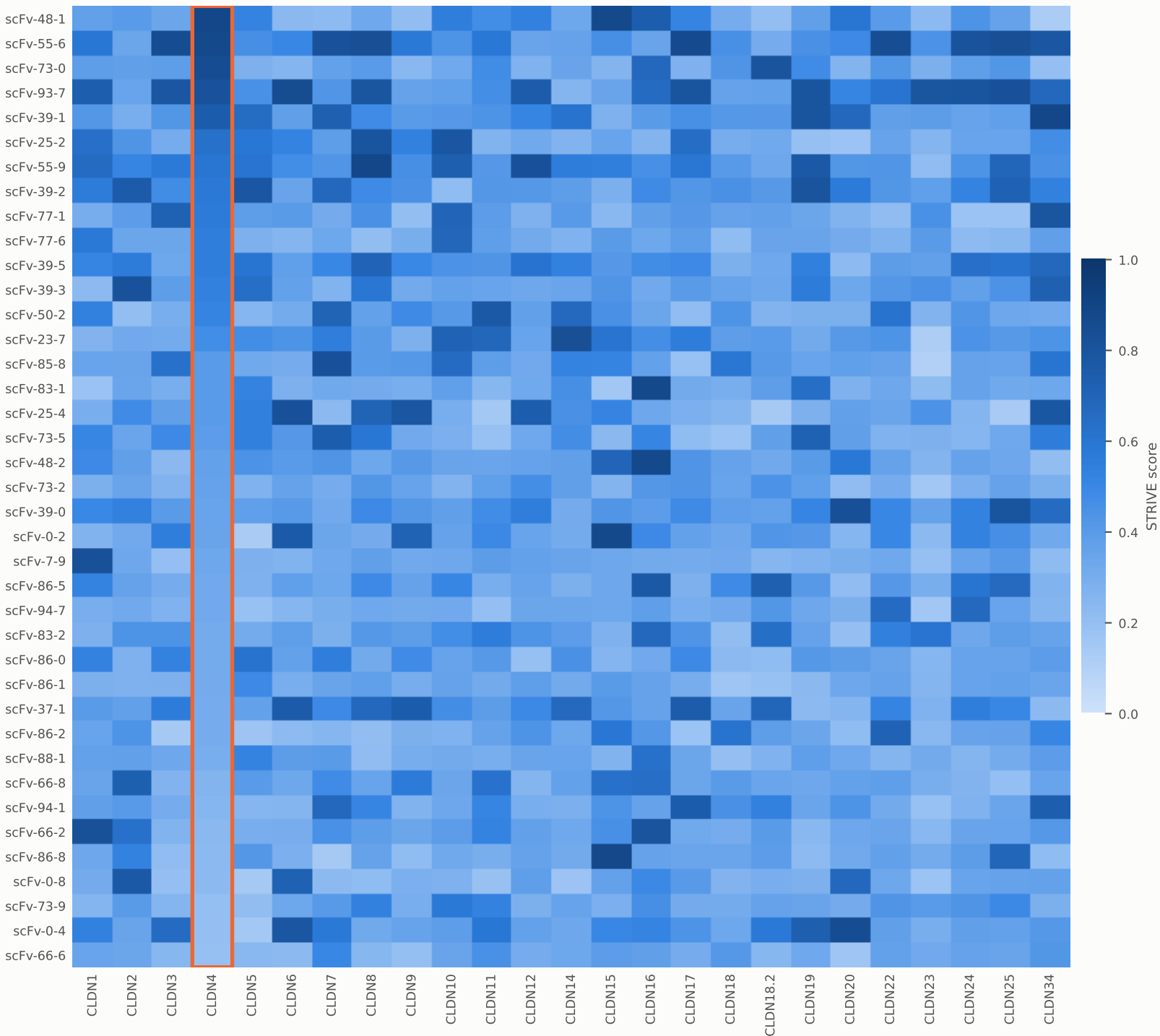
Predicted cross-reactivity landscape: 39 candidates × 25 antigens (CLDN4 on-target column outlined)
