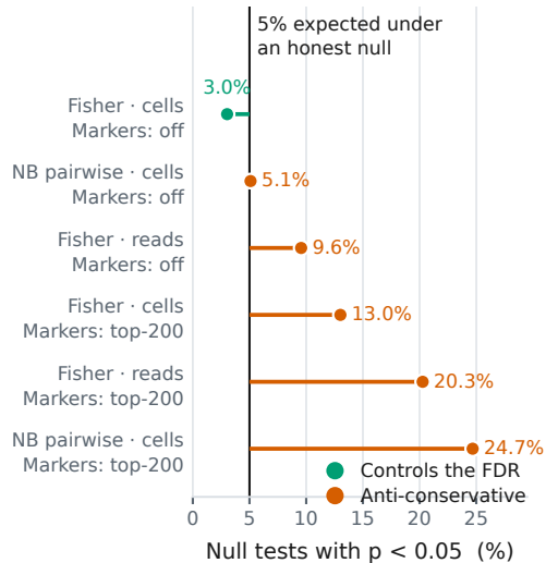
a False-positive rate
