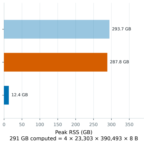
d Where the memory went — profiling, not peak calling
