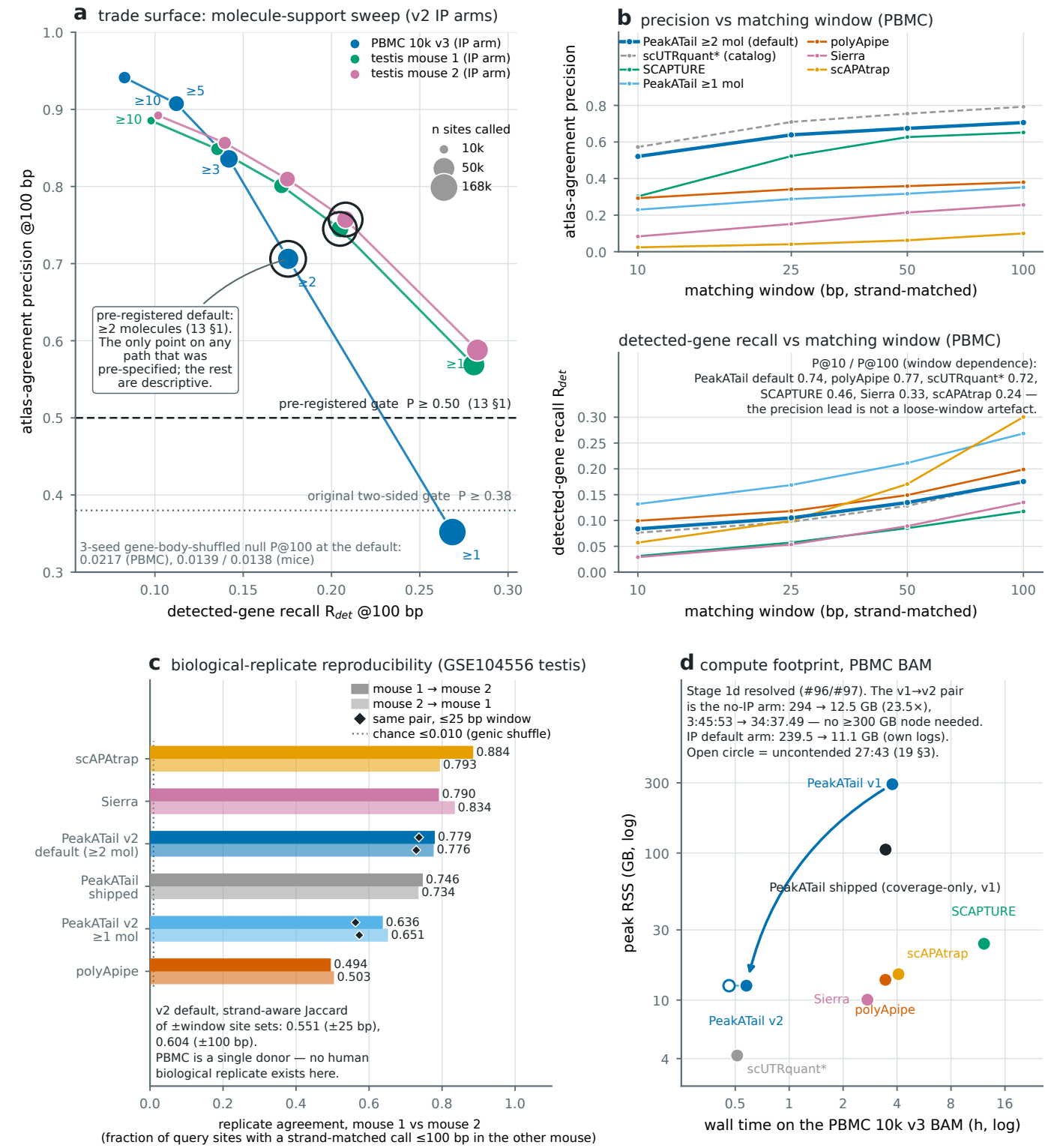
Fig 3 | Operating-point trade surface, window sensitivity, replicate reproducibility and compute
