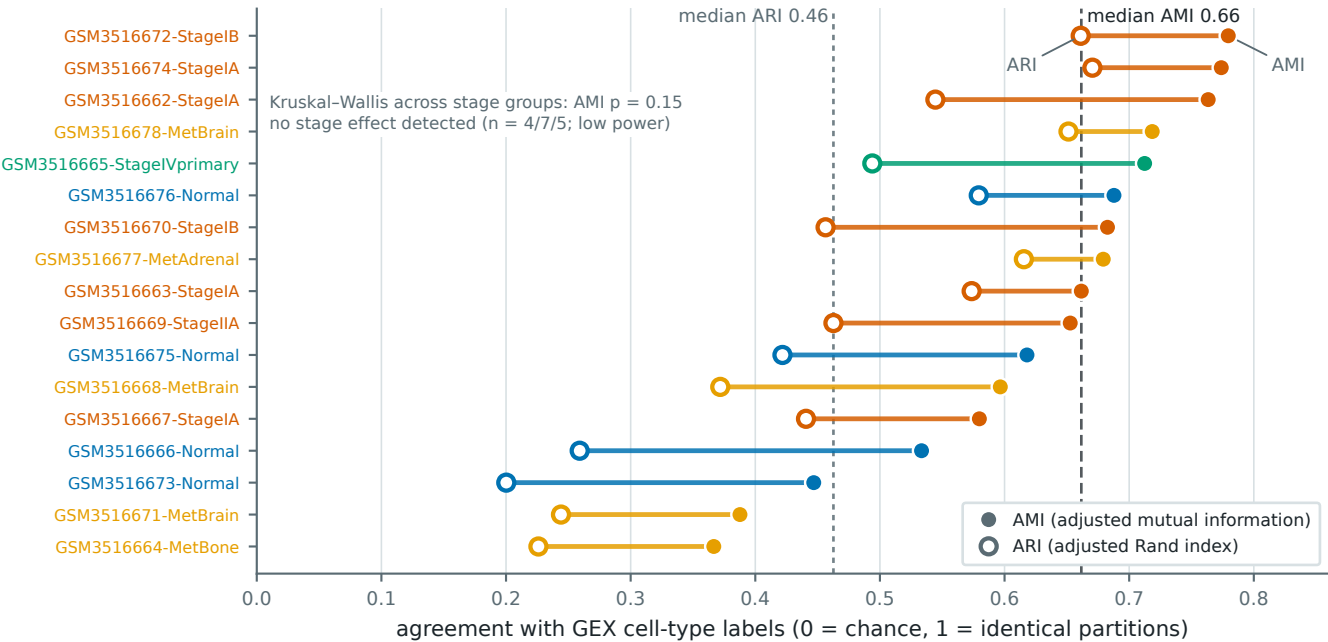
b PAS space finds structure of the same granularity, slightly finer
