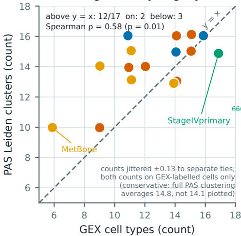
b PAS space finds structure of the same granularity, slightly finer
