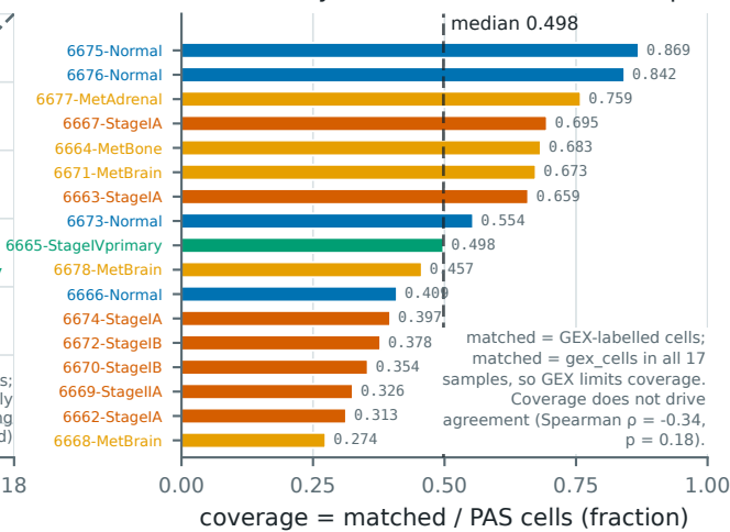
c Caveat: concordance is scored on a minority of PAS cells in 9 of 17 samples
