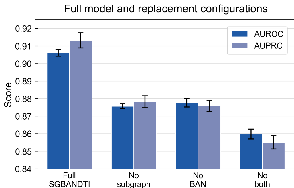
Figure 2. Architecture-replacement analysis on the BioSNAP random split. The figure compares AUROC and AUPRC across the full model and three replacement configurations; error bars denote the sample standard deviation ( n = 5 training seeds). Replacing rooted subgraphs or bilinear attention produces similar degradation, and replacing both components yields the largest loss.
