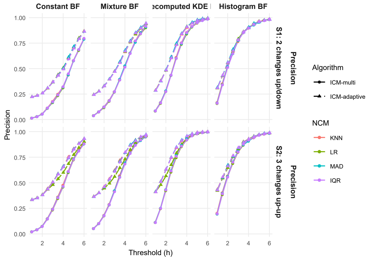
comparison by BF and Algorithm
