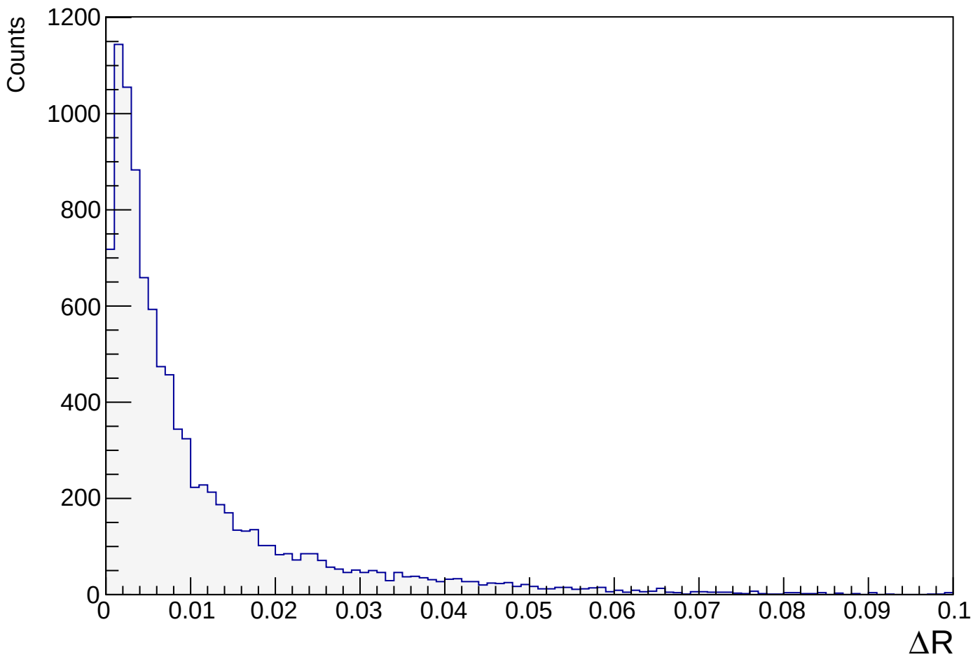
\Delta R between the generated and matched photons
