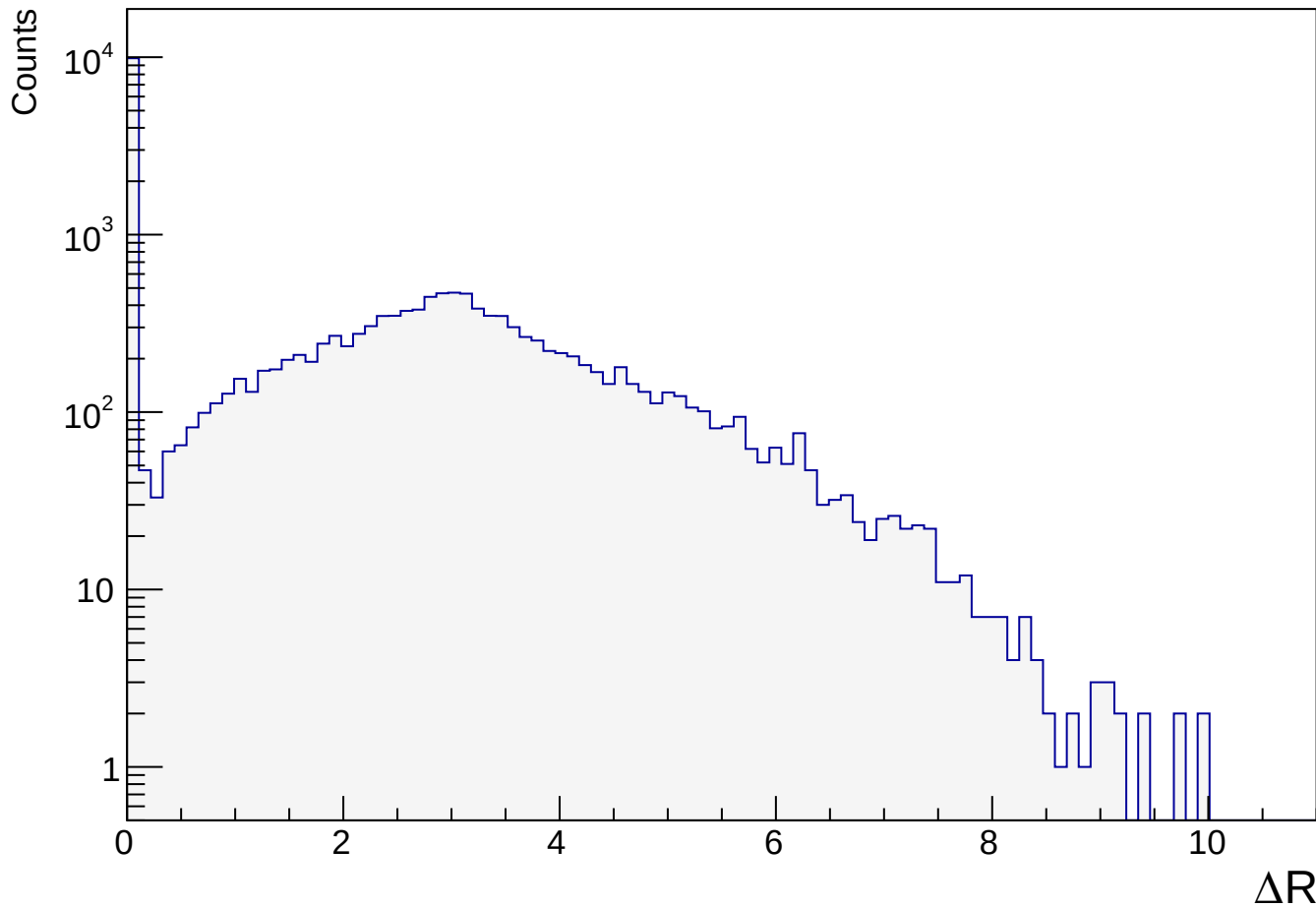
\Delta R between the generated and matched photons
