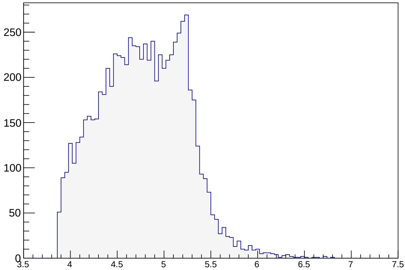
candBsMass
