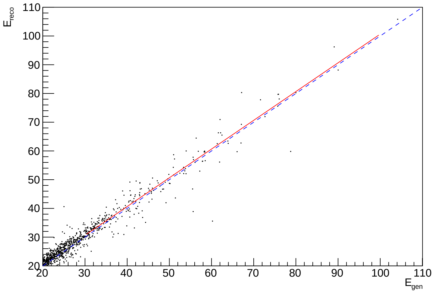
EB_p0_ Photon energy
