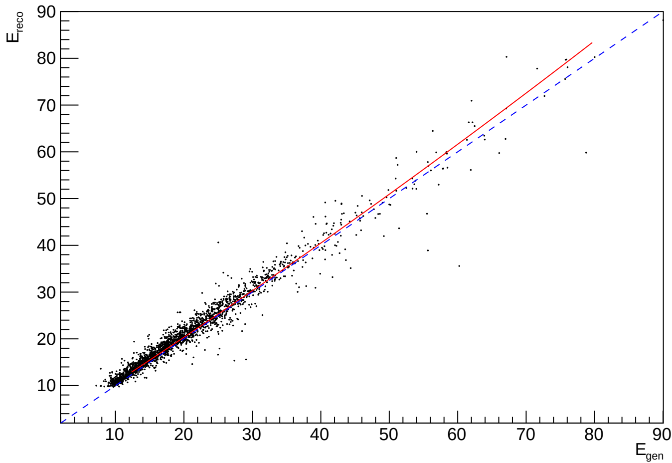
EB_p2_ Photon energy
