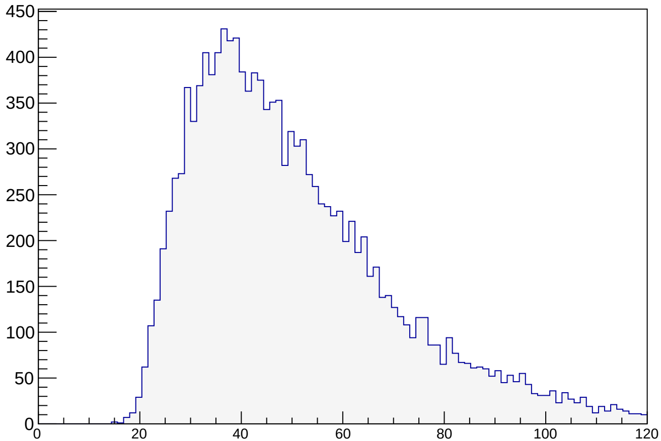
candBsPt
