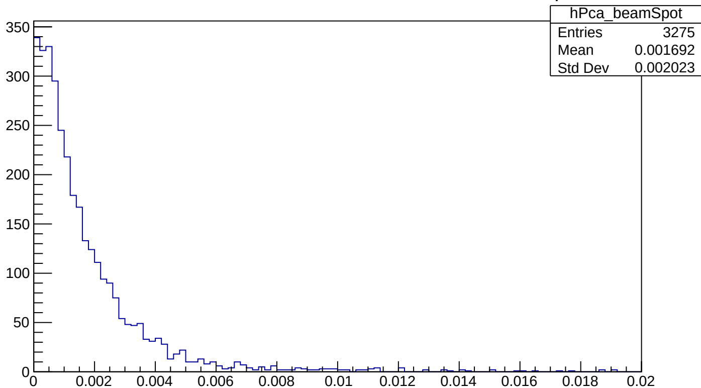
Distance of the fitDimuonRecoPhotonMomentum to beamSpot
