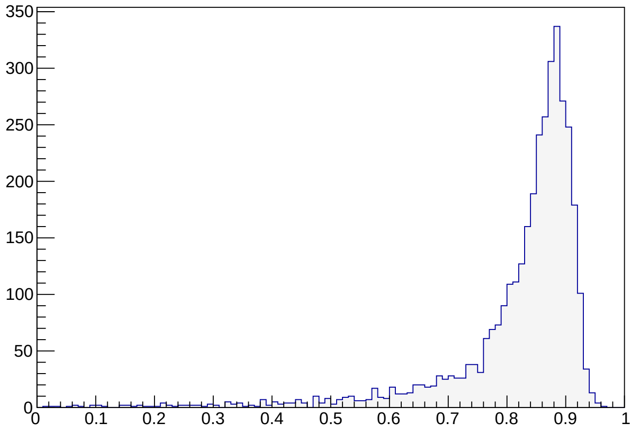
Muon Id score
