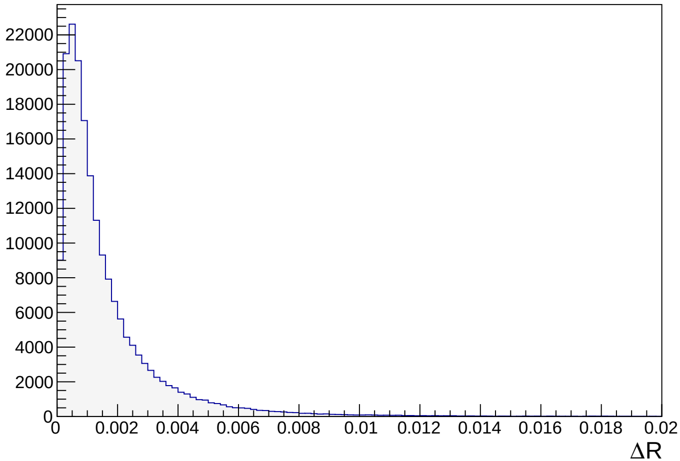
\Delta R between the generated and matched muons
