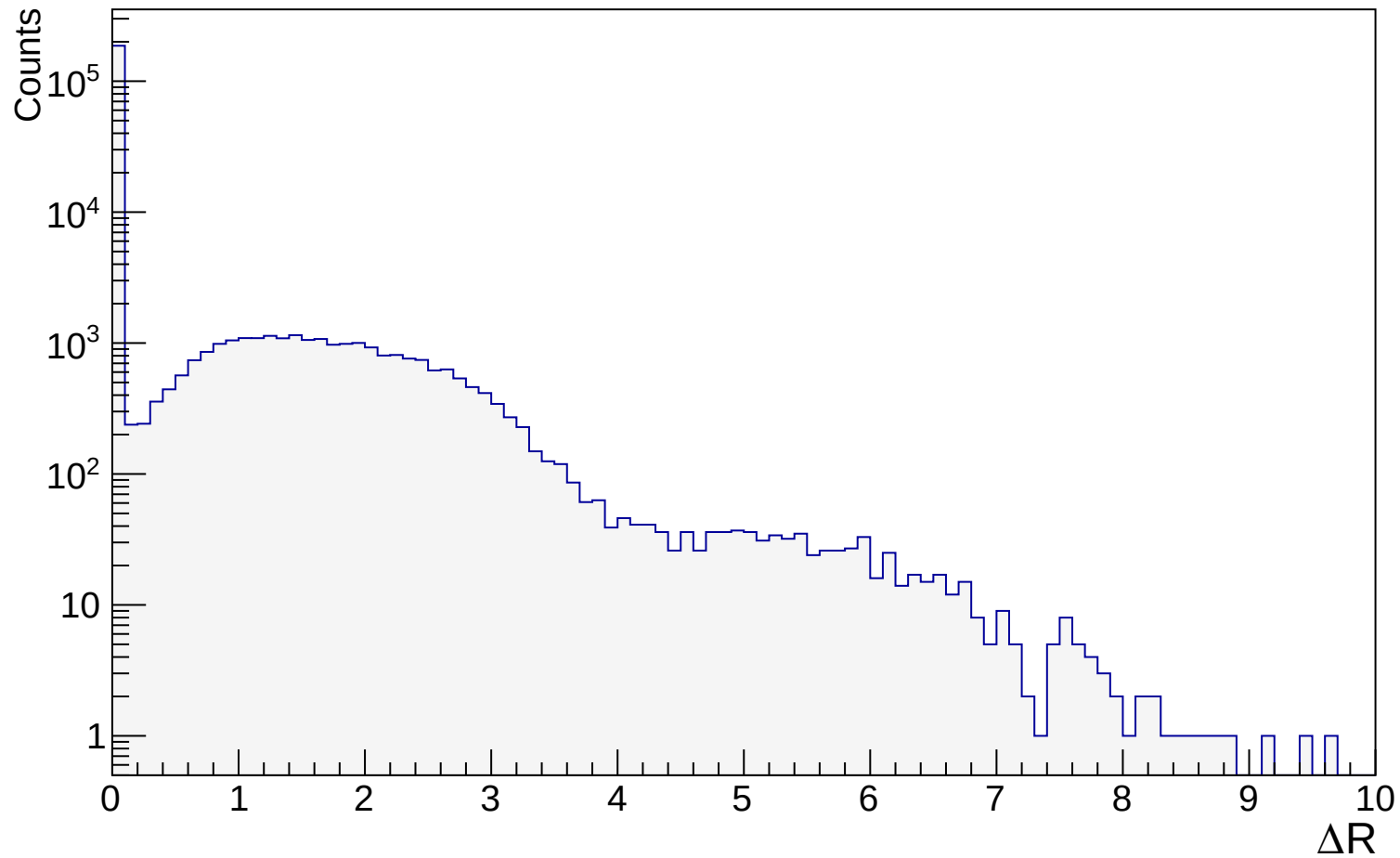
\Delta R between the generated and matched muons
