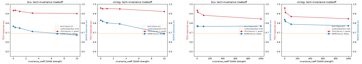
Figure 6: Technology-vs-biology trade-off. Left: DANN — biology is lost \sim 3\times faster than technology; no sweet spot. Right: CORAL — technology drops while biology stays essentially flat (a clearly favorable trade), but only the linear leak is removed. [M]
