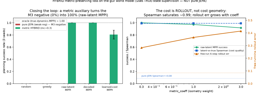
Figure 5: The isometry auxiliary closes the planning loop: pure JEPA 0% vs. HYBRID 100% at oracle quality, with latent \leftrightarrow true rank correlation 0.085 \rightarrow 0.990 . [M]
