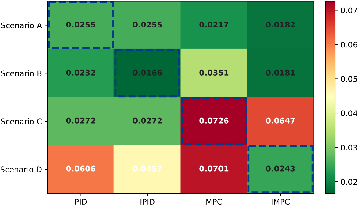
Velocity tracking RMSE (m/s) lower is better | dashed = engineered winner
