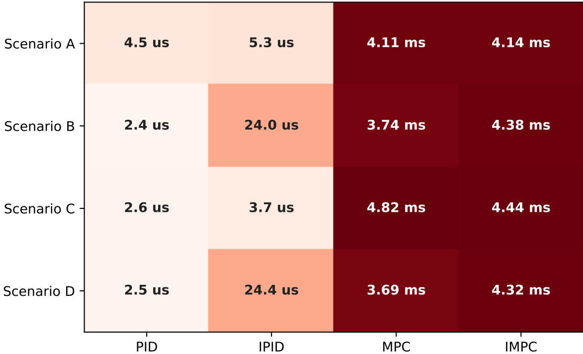
Mean compute per controller tick lower is better | log colour scale
