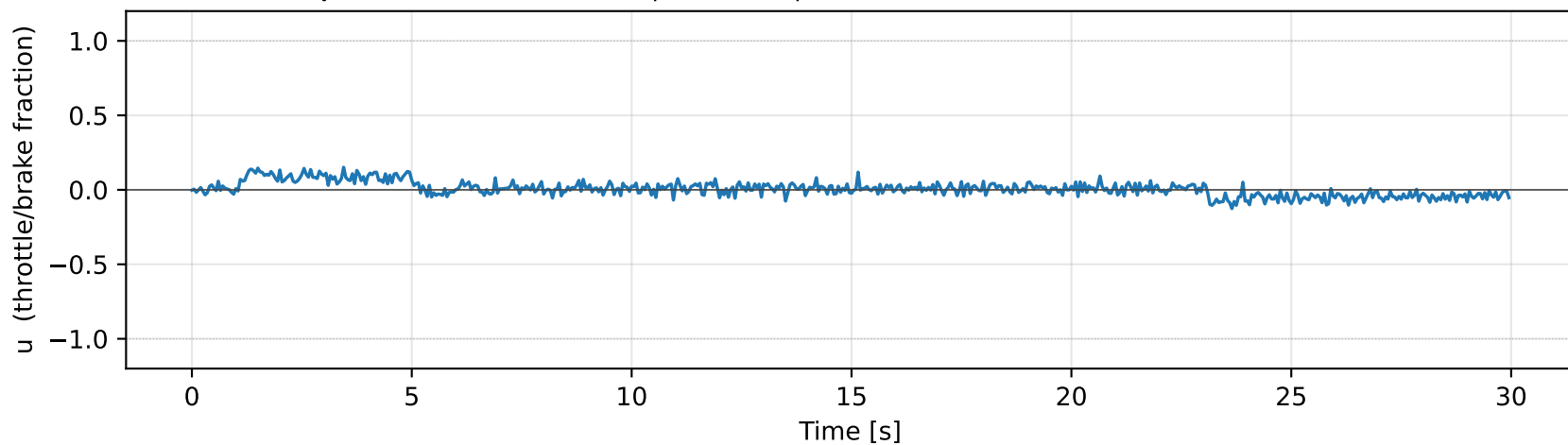
Control effort ( \int u^2 dt = 0.075 , mean compute = 2.8 \mu s)
