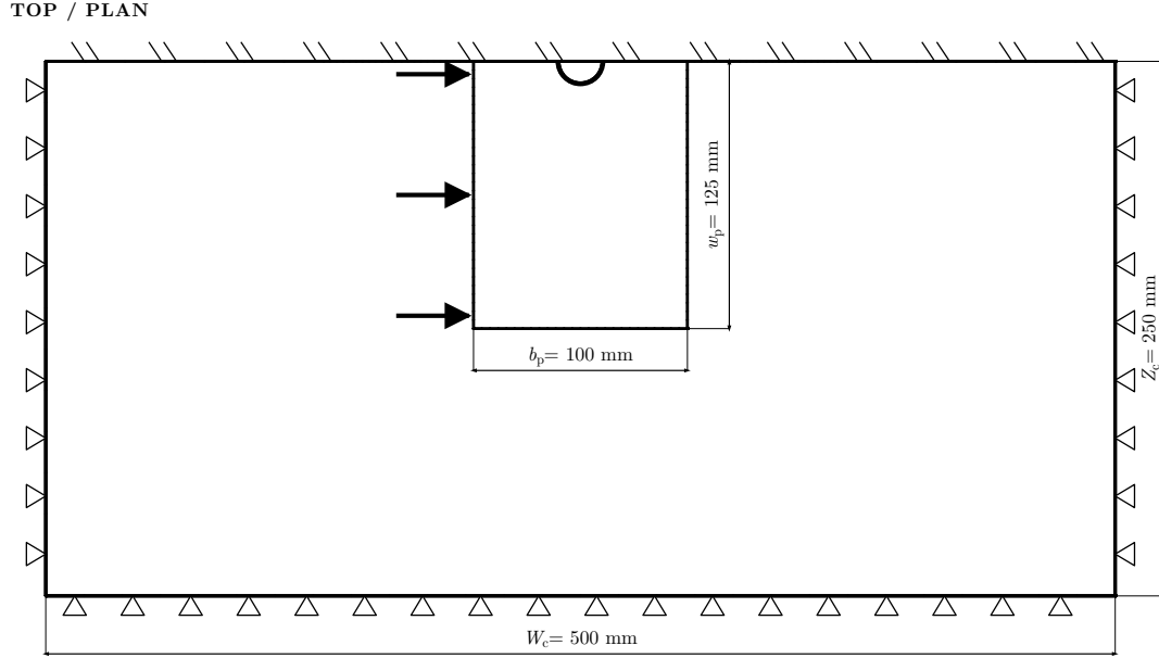
Figure 6: Top view of the model including the plane of symmetry z = 0 , across which the model and the loading are symmetric. The prescribed displacement u_x = 5 mm is distributed over the 32 nodes of the plate edge set plate_left_loading .
