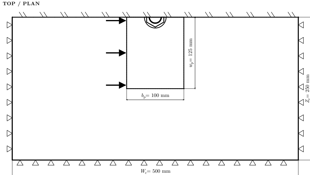
Figure 2: Top view of the model including the plane of symmetry z = 0 , across which the model and the loading are symmetric. The prescribed displacement u_x = 5 mm is distributed over the 32 nodes of the plate edge set plate_left_loading .
