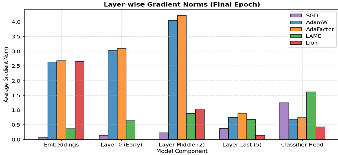
Figure 5.4: Detailed layer-wise gradient norm comparison at Epoch 3.
