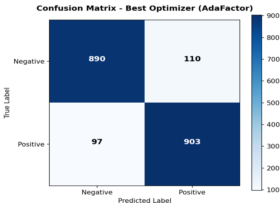
Figure 5.6: Confusion matrix on the IMDB test set for the recommended optimizer (AdaFactor).
