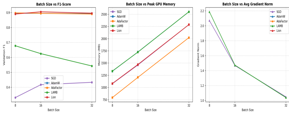
Figure 5.8: Batch size robustness curves showing validation F1 -score, peak GPU memory, and gradient norm.
