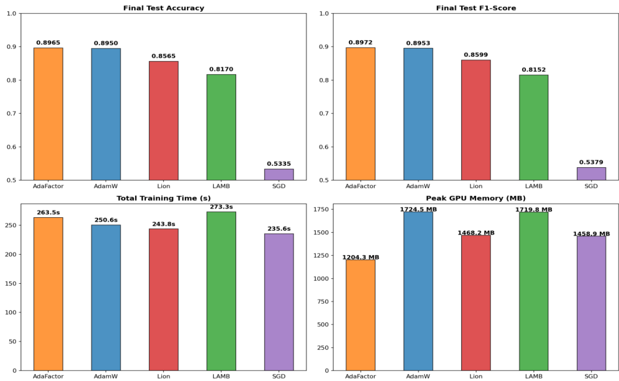
Figure 5.5: Bar charts comparing test accuracy, F1-score, training time, and peak GPU memory.
