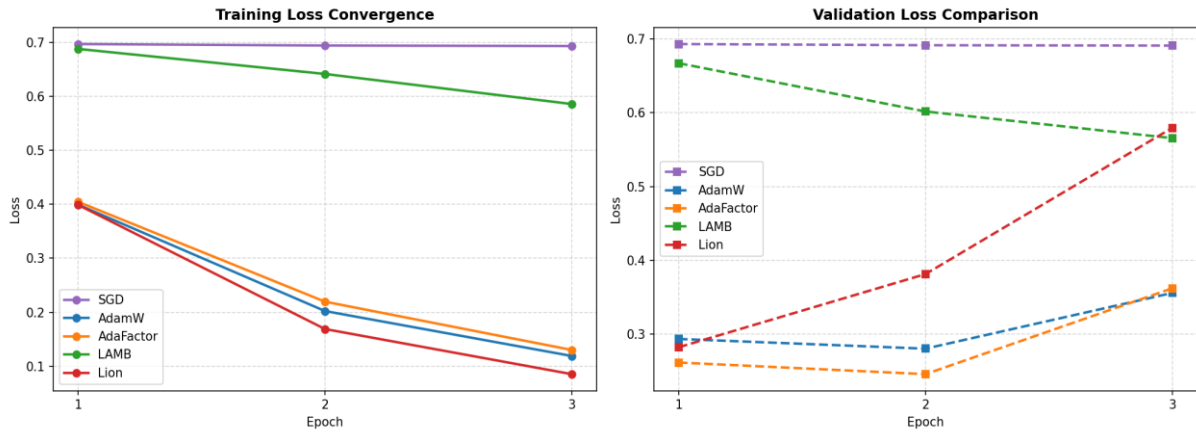
Figure 5.1: Training and validation loss curves over the three training epochs.
