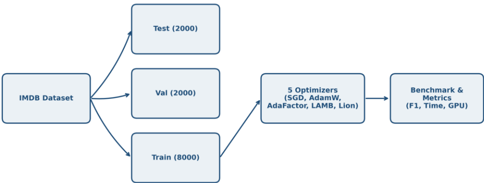
Figure 1.2: Experimental pipeline outlining dataset splitting, multi-optimizer benchmarking, and metric extraction.
