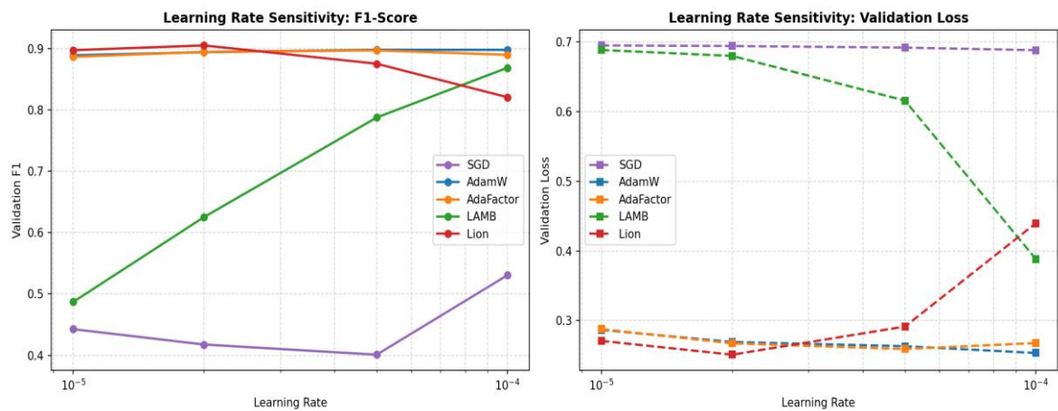
Figure 5.7: Learning rate sensitivity curves showing validation F1-score (left) and validation loss (right).
