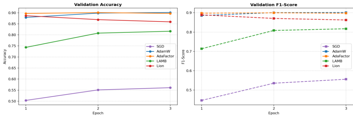
Figure 5.2: Validation accuracy (left) and F1-score (right) trajectories across epochs.
