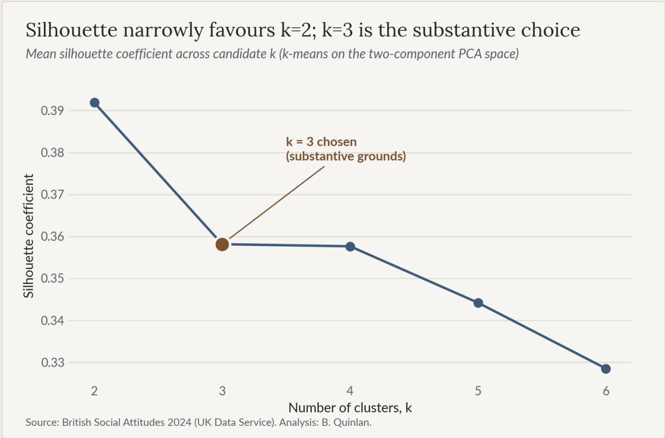
Figure 4. Silhouette scores across candidate k; k=3 is adopted on substantive grounds.
