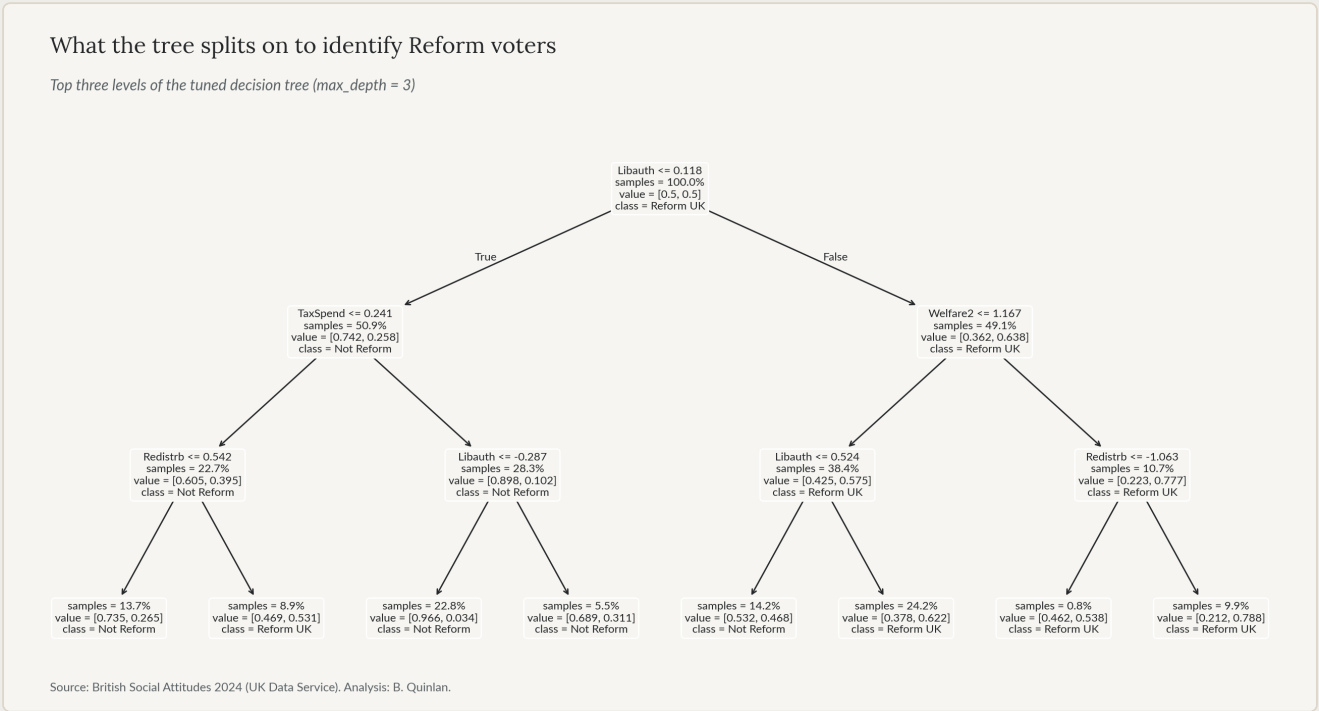
Figure 11. The top of the tuned decision tree, showing its principal splits.
