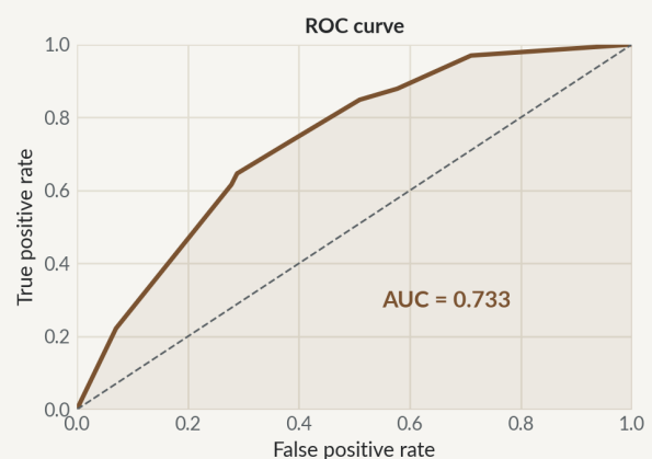
Figure 10. A supervised decision tree separates Reform voters with moderate accuracy (AUC ≈ 0.73).
