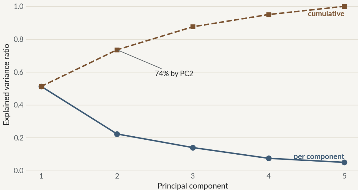
Figure 2. Two principal components retain roughly three-quarters of the attitudinal variance.
