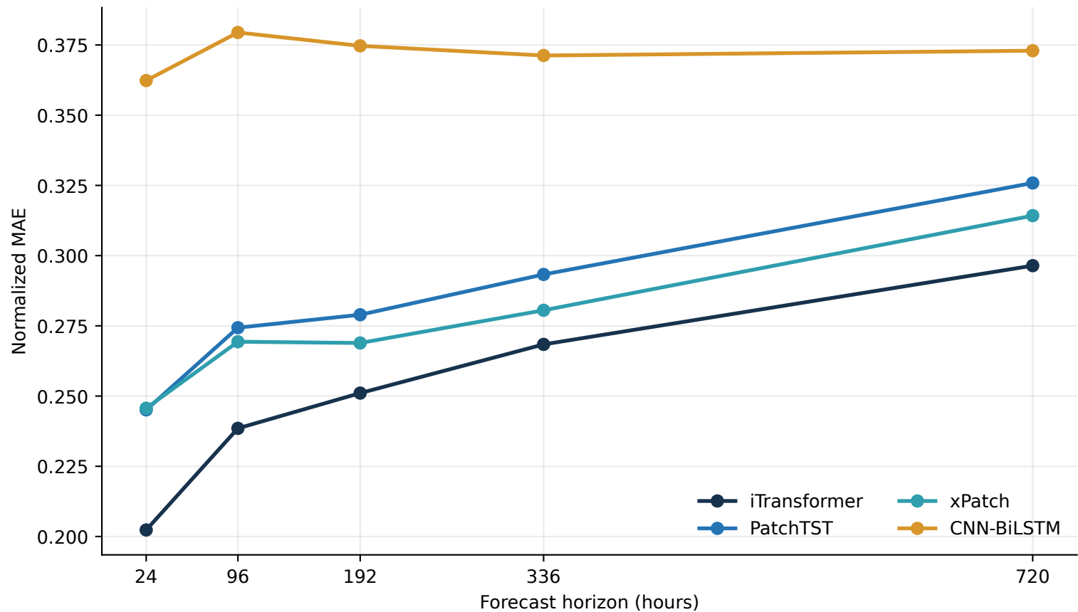
ECL benchmark: normalized MAE increases with forecast horizon
