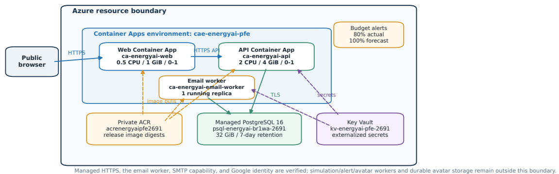
Figure 6.12 – Verified Azure deployment topology for Product V1. Solid arrows show runtime traffic; dashed arrows show image or secret supply.
