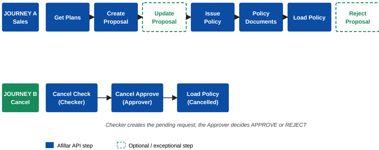
Figure 2: Insurance API orchestration flows — Sales (Journey A) and Cancellation (Journey B)
