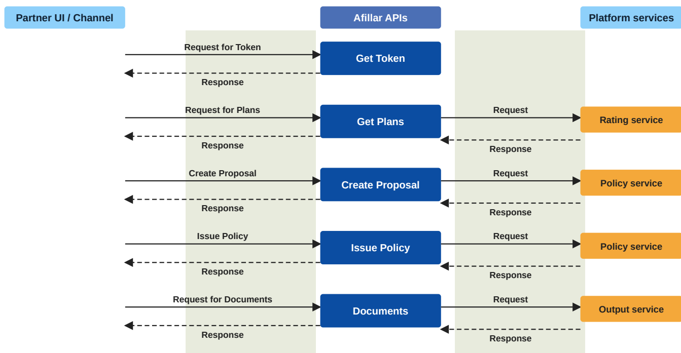
Figure 1: Sales journey — sequence across the channel, the APIs and the platform
