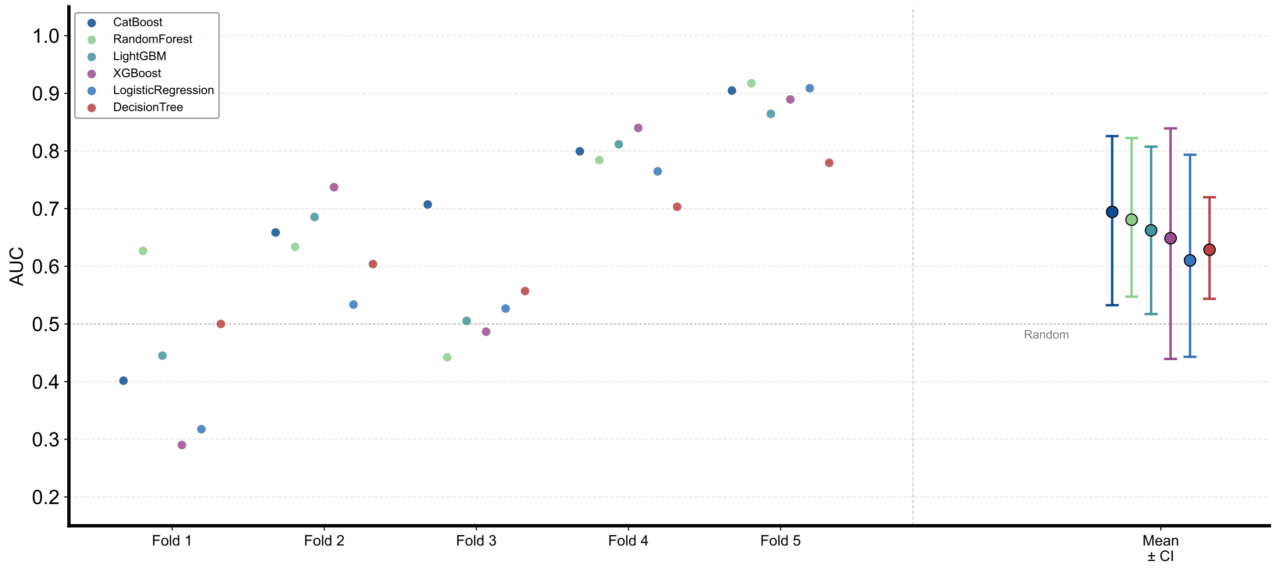
Per-Fold AUC with Mean \pm Bootstrap CI (TimeSeriesSplit 5-Fold)
