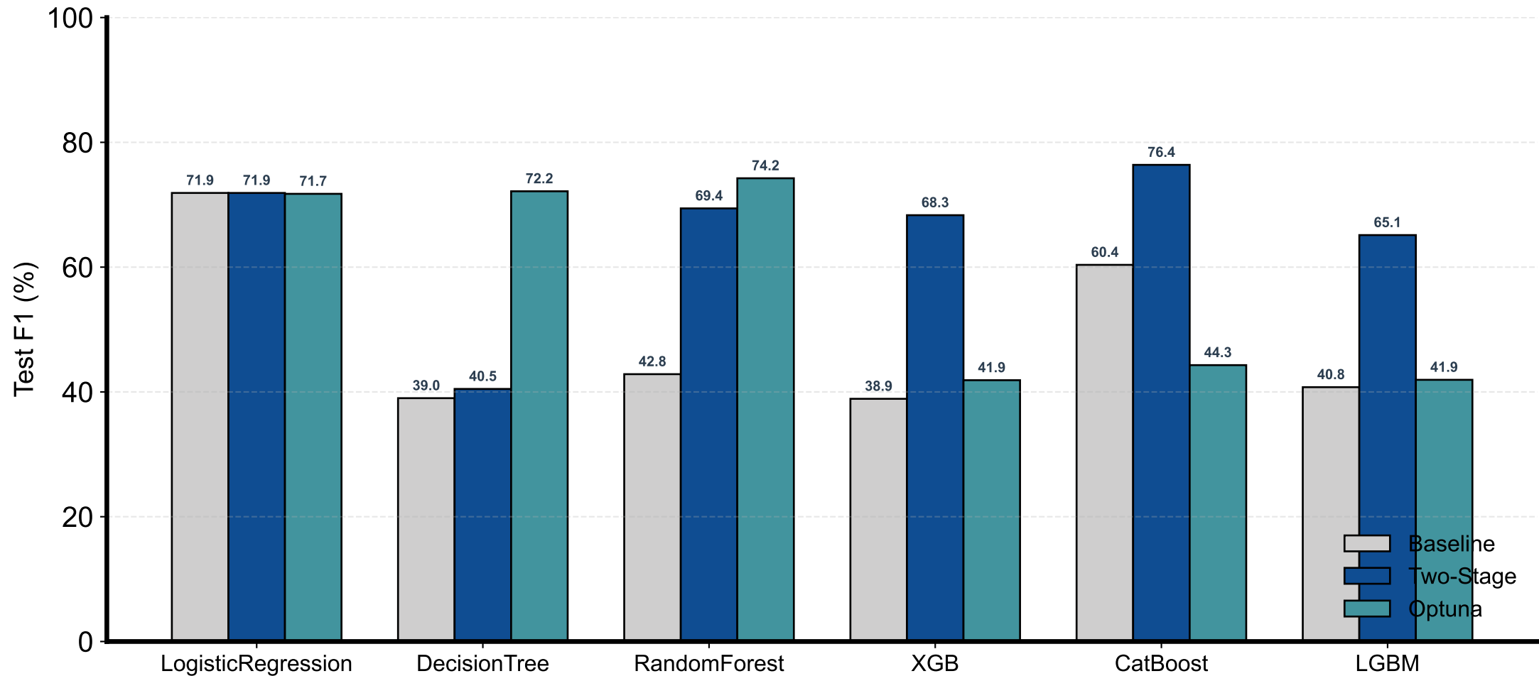
Model F1 Comparison: Baseline vs Two-Stage vs Optuna
