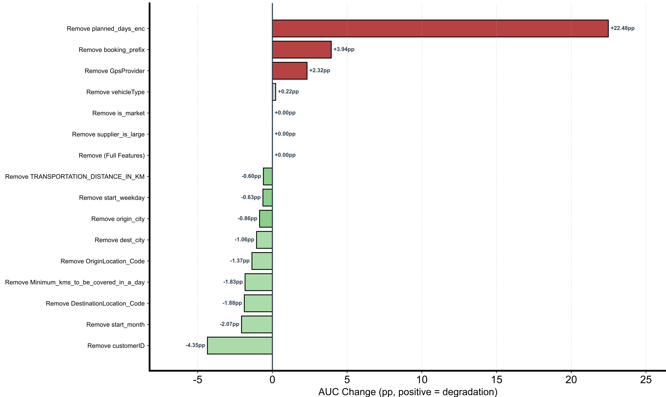
Feature Ablation — CatBoost Leave-One-Out (Temporal Split)
