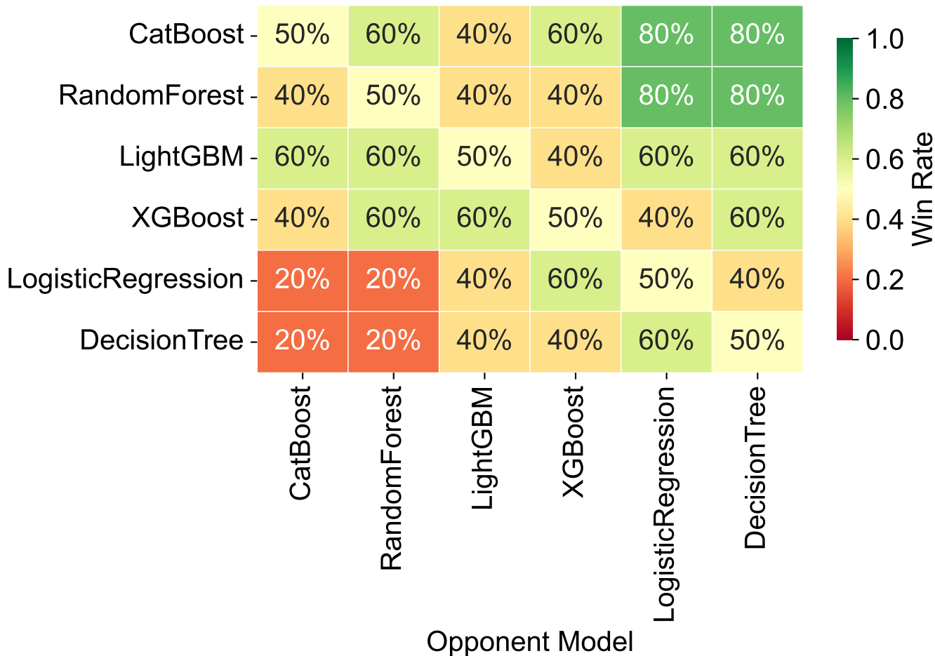
Pairwise Win Matrix (TimeSeriesSplit 5-Fold)
