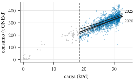
Fuel gás
