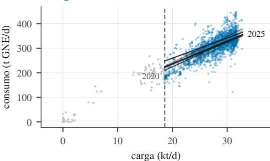
Fuel gás
