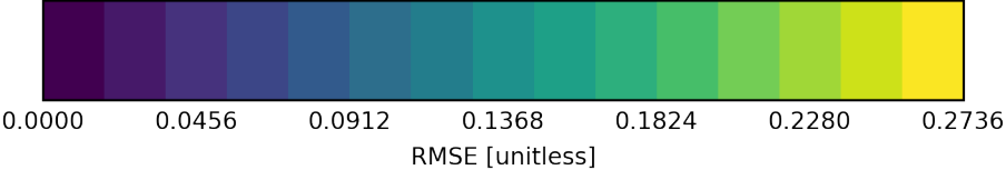
Heatmap RMSE (Summary) nasa-aeronet/directsun_v3-lev15|od550aero
