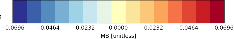
Heatmap MB (Summary) nasa-aeronet/directsun_v3-lev15|od550aero
