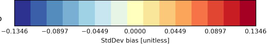
Heatmap StdDev bias (Summary) nasa-aeronet/directsun_v3-lev15|od550aero
