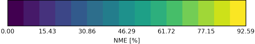
Heatmap NME (Summary) nasa-aeronet/directsun_v3-lev15|od550aero
