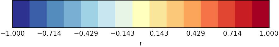
Map r (Summary) nasa-aeronet/directsun_v3-lev15|od550aero
