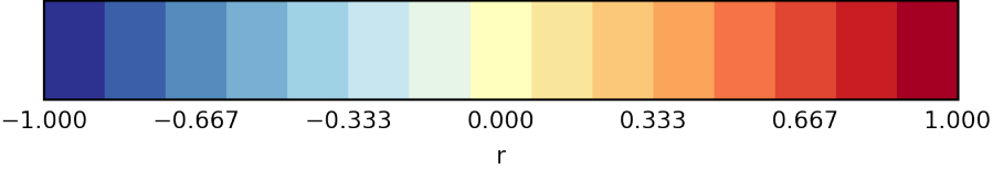
Heatmap r (Summary) nasa-aeronet/directsun_v3-lev15|od550aero
