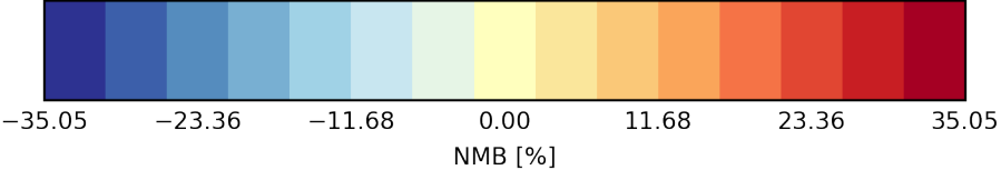
Heatmap NMB (Summary) nasa-aeronet/directsun_v3-lev15|od550aero
