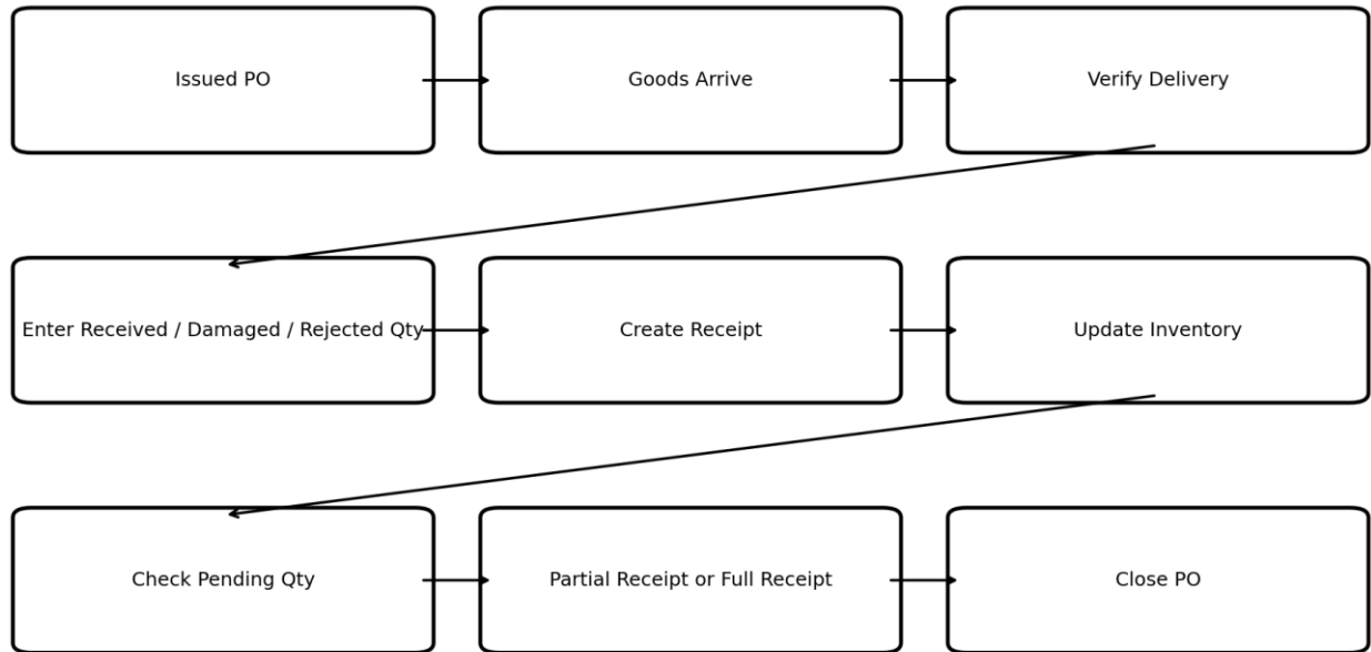
Figure 6. Goods receiving and inventory update flow.
