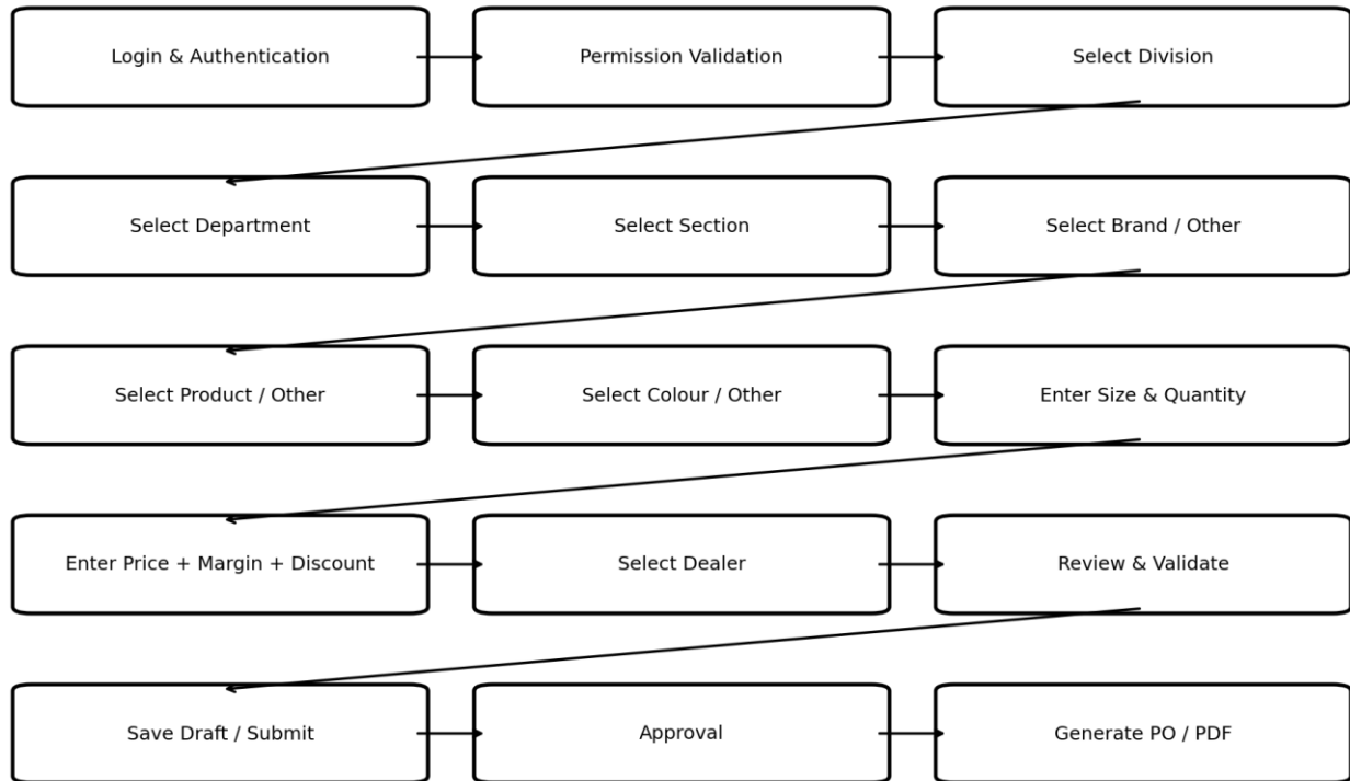
Figure 4. Guided purchase entry workflow.
