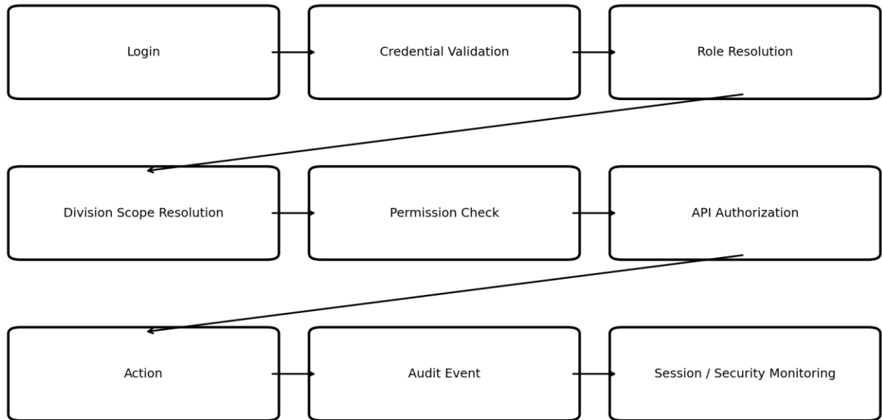
Figure 3. Security and authorization flow.
