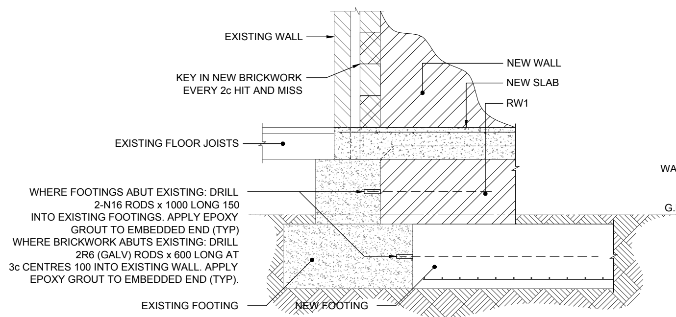
DETAIL E 1:20
