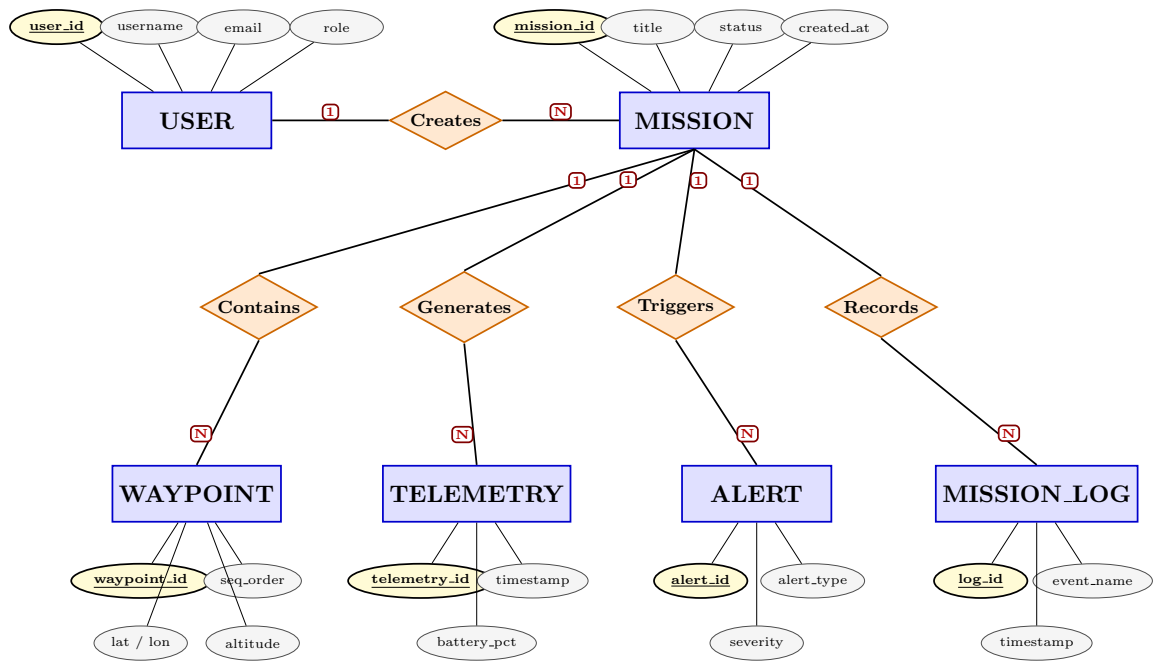
Figure 1: Entity-Relationship (ER) Diagram for Astra Command PostgreSQL Database
