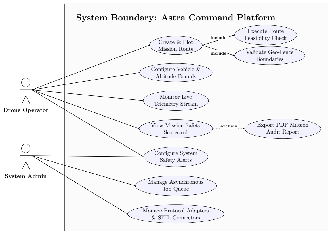
Figure 1: UML Use Case Diagram for Astra Command Platform
