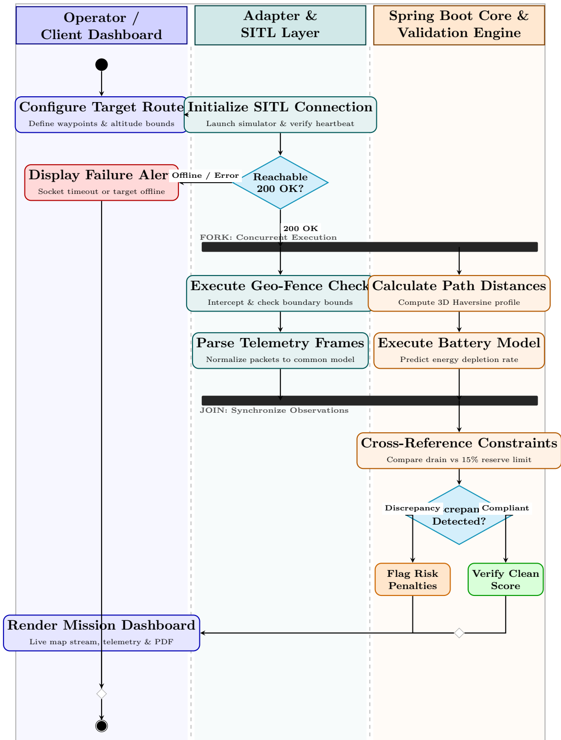
Figure 1: UML Swimlane Activity Diagram for Astra Command Platform Execution
