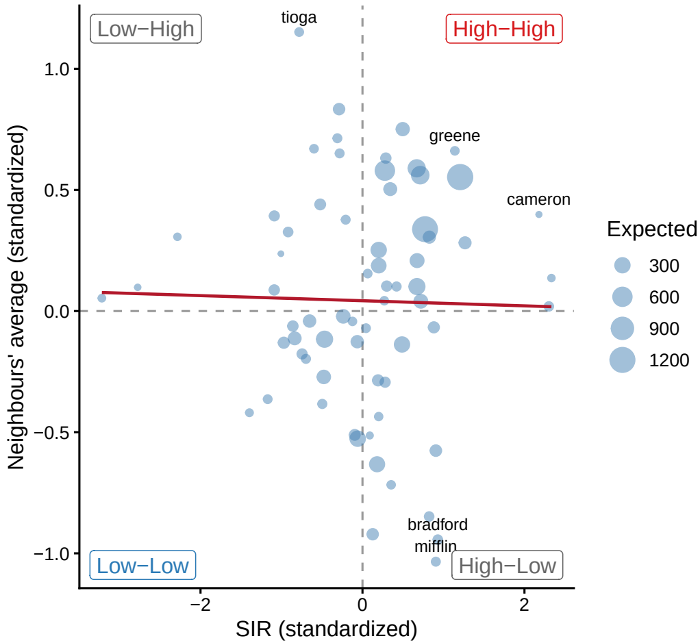
Figure 4: Moran scatterplot. The slope of the line is Moran's I.
