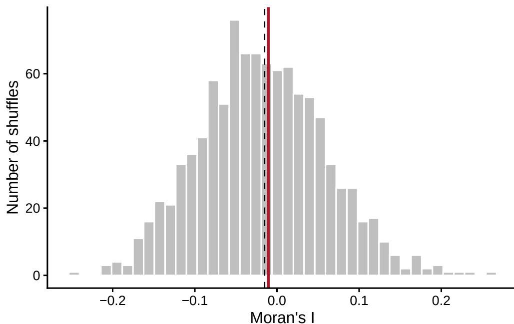
Figure 6: Moran's I under 999 random shufflings (grey) and the observed value (red).
