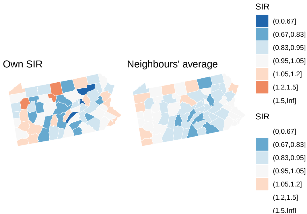
Figure 3: Each county's own SIR (left) and the average SIR of its neighbours (right).
