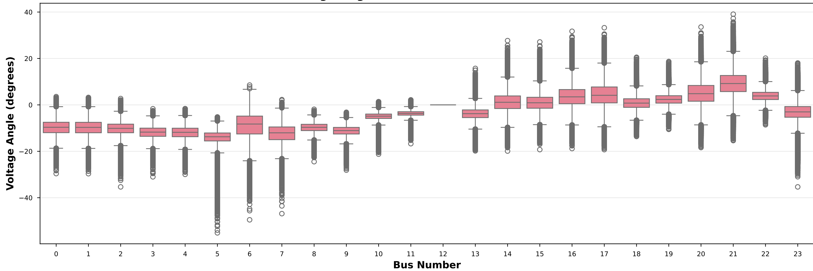
Voltage Angle Distribution Across All Buses
