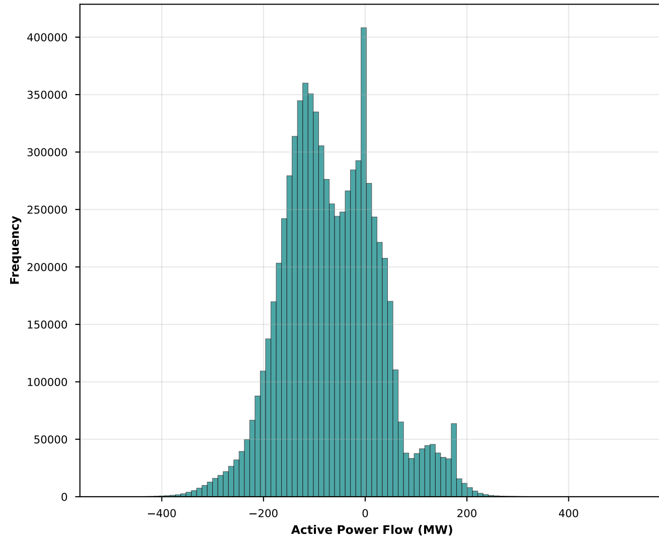
Branch Active Power Flow Distribution
