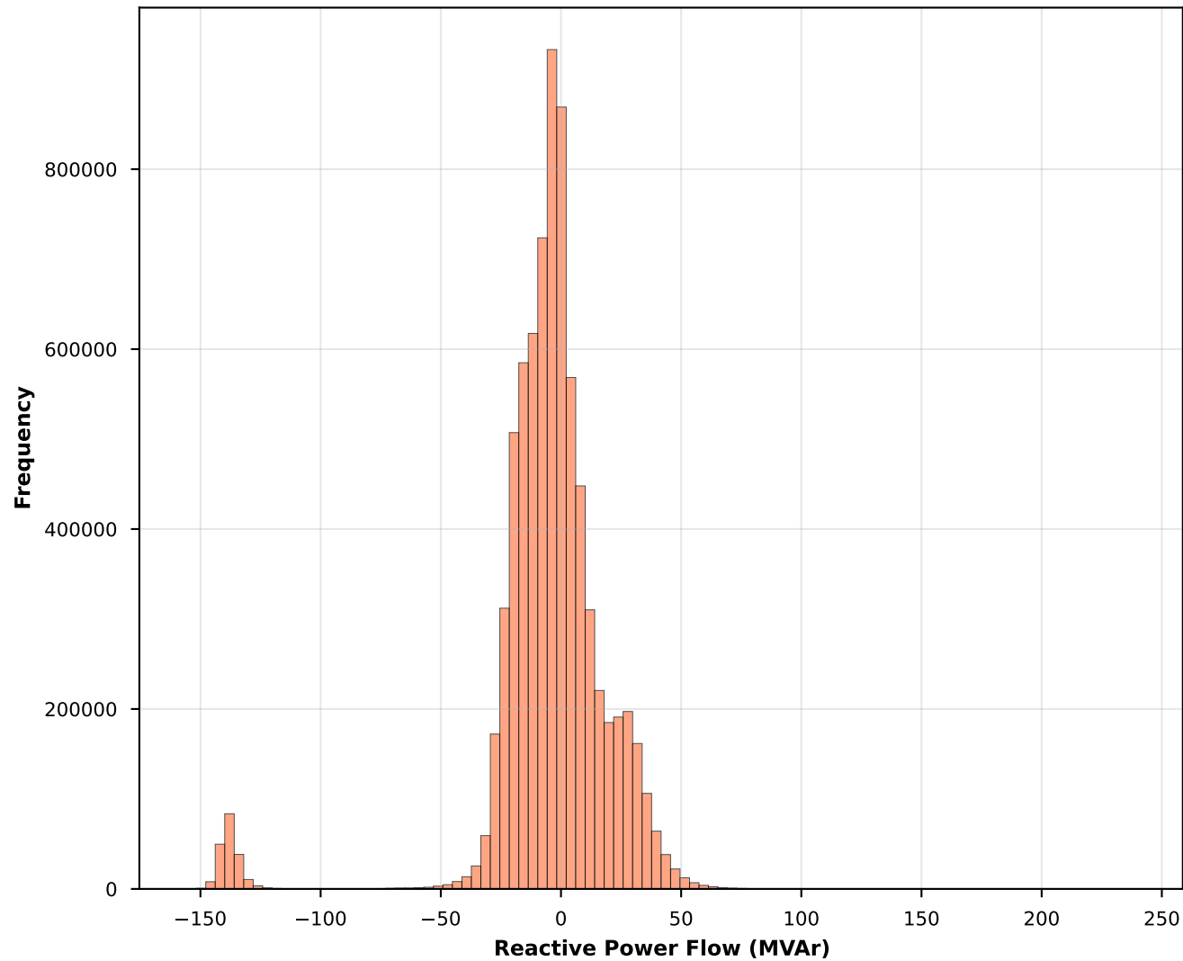
Branch Reactive Power Flow Distribution
