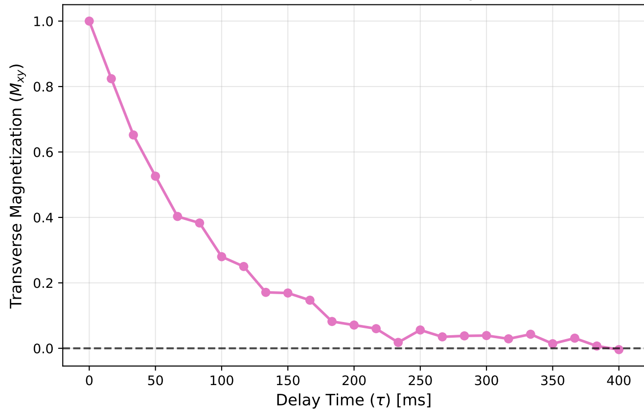
Quantum Simulation: Free Induction Decay ( T_2 Relaxation)
