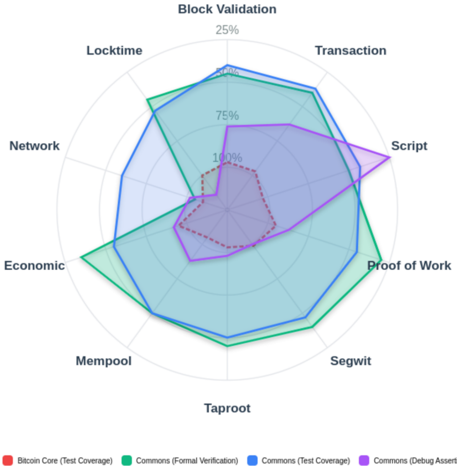
Figure: Consensus coverage comparison: Bitcoin Core achieves coverage through testing alone. Bitcoin Commons achieves formal verification coverage (Kani proofs) plus comprehensive test coverage. Commons uses consensus-focused test files with extensive test functions compared to Core's total files. The mathematical specification enables both formal verification and comprehensive testing.
