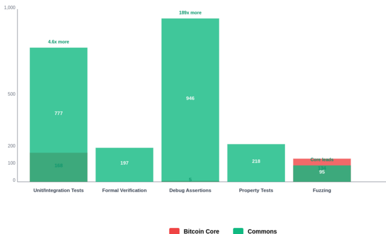
Figure: Comparison of verification methods: Bitcoin Core relies primarily on unit/integration tests and fuzzing. Bitcoin Commons employs comprehensive formal verification, extensive test coverage, debug assertions, and property tests, providing multiple layers of verification beyond Core's approach.
