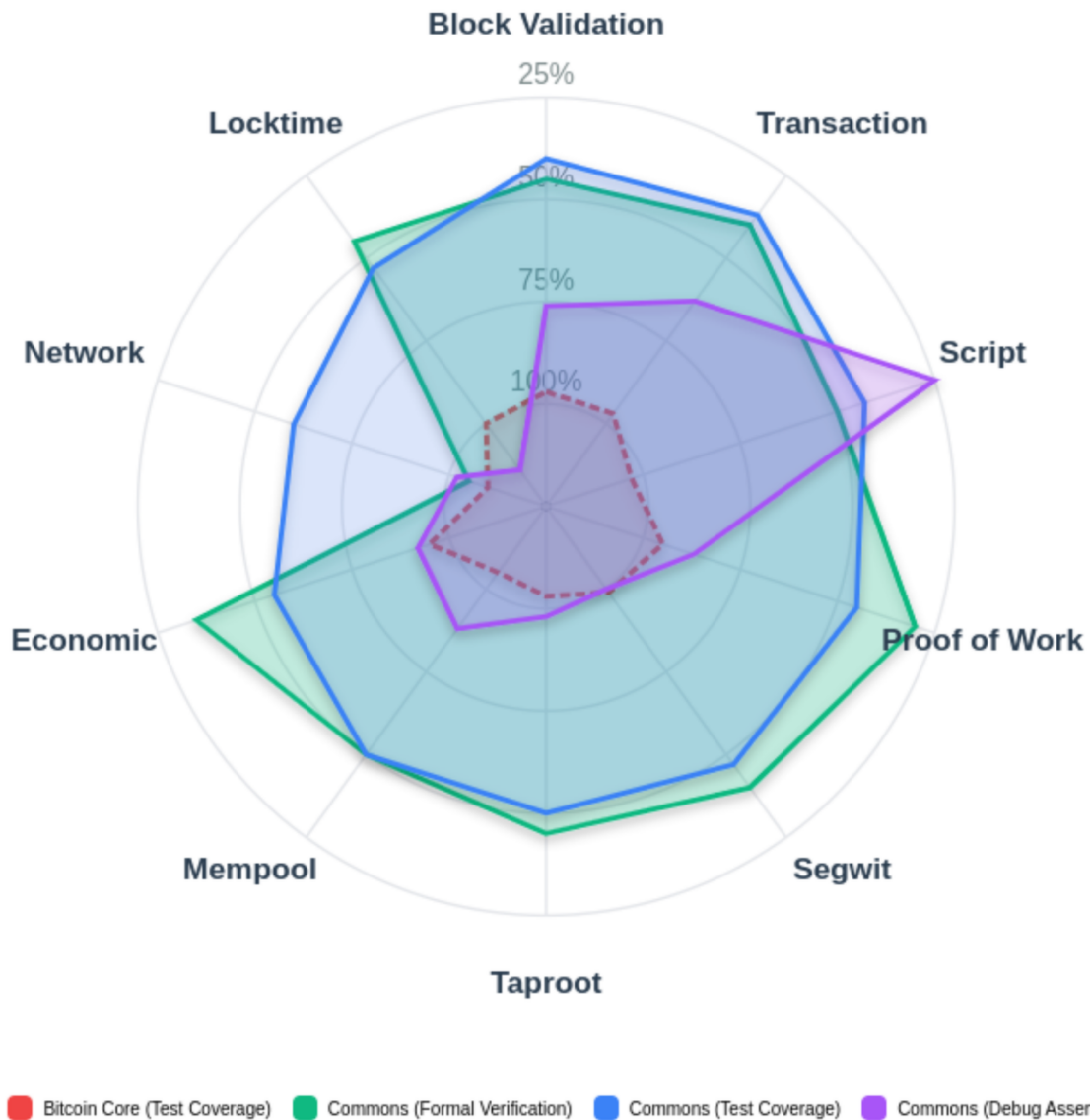
Figure: Consensus coverage comparison: Bitcoin Core achieves coverage through testing alone. Bitcoin Commons achieves formal verification coverage (Kani proofs) plus comprehensive test coverage. Commons uses consensus-focused test files with extensive test functions compared to Core's total files. The mathematical specification enables both formal verification and comprehensive testing.
