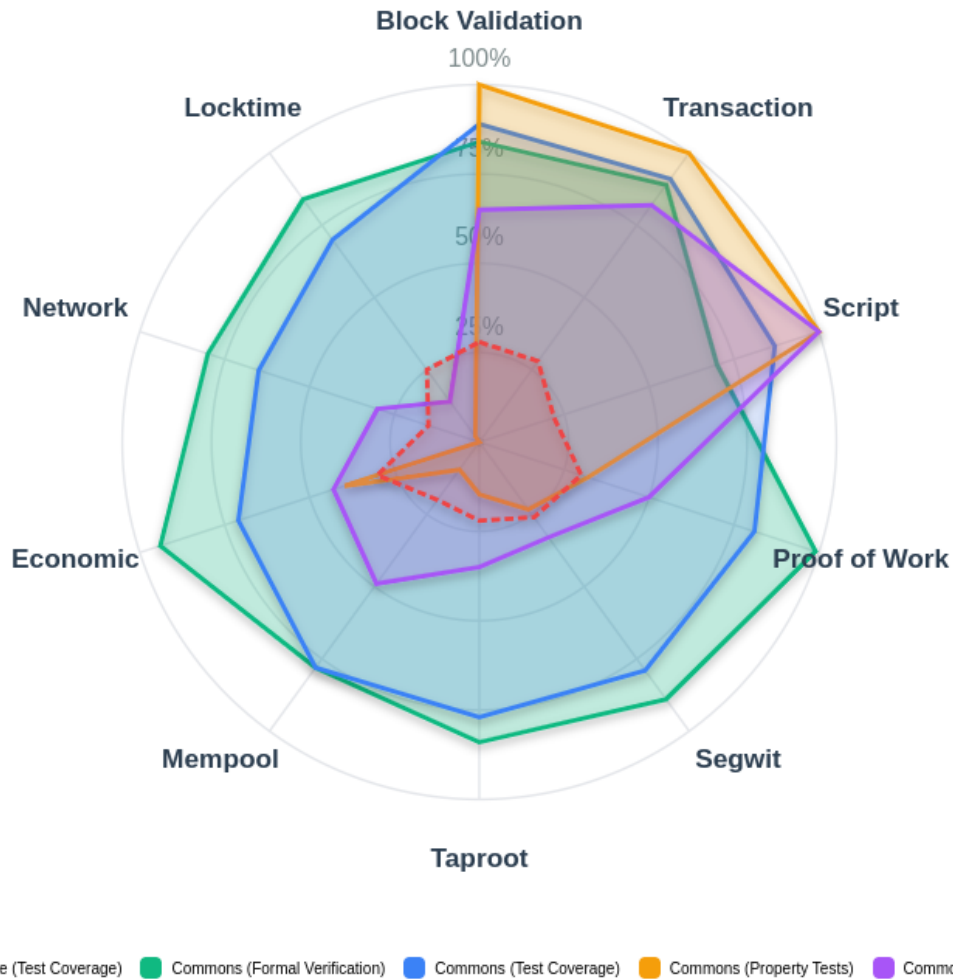
Figure: Consensus coverage comparison: Bitcoin Core achieves coverage through testing alone. Bitcoin Commons adds spec-lock verification (contracts plus Z3-backed checks where enabled) on top of comprehensive test coverage. Commons uses consensus-focused test files with extensive test functions compared to Core's total files. The mathematical specification enables both machine-checked contracts and testing.
