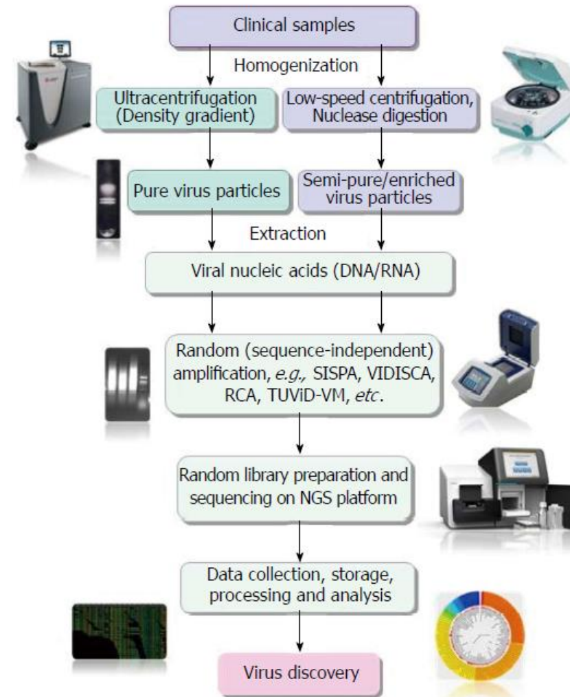
Figure 1 Diagrammatic representation of main steps of clinical virus discovery by next-generation sequencer based technologies.
