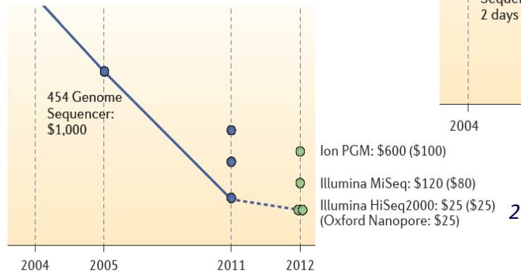
Cost per Mb assembled sequence
