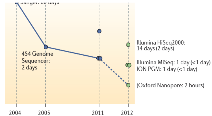
Turnaround time: bacterial genome
