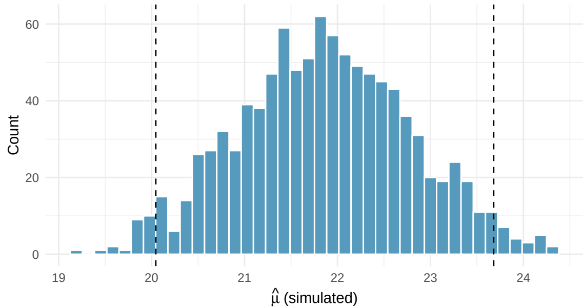
Simulated sampling distribution of \mu -hat
