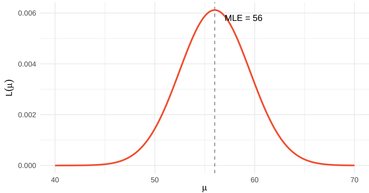
Likelihood for the Temperature Example ( x_1 = 55 , x_2 = 57 )
