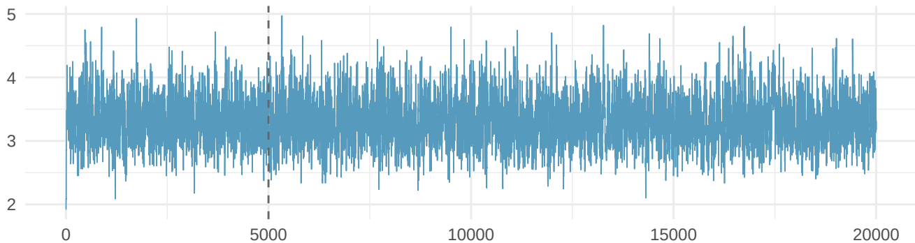
r (dispersion)
